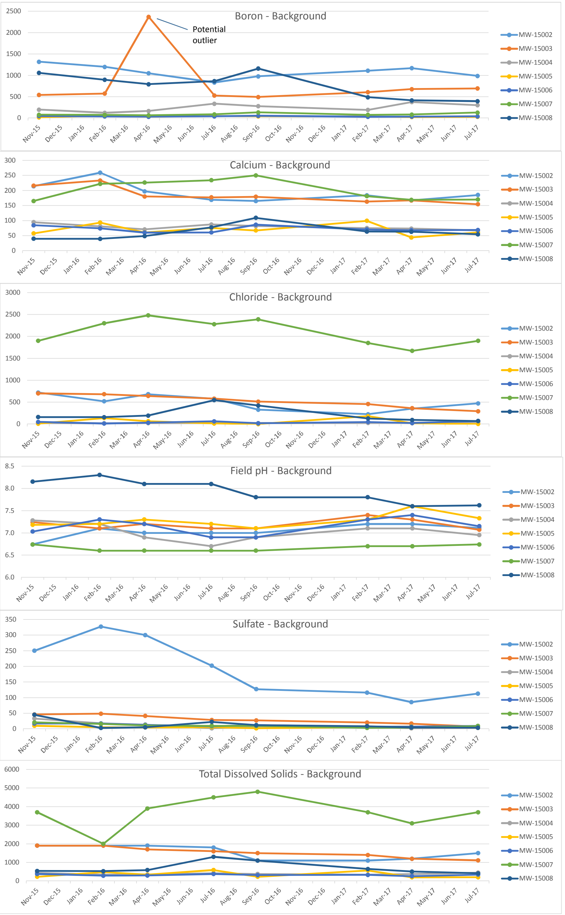
Figure 1 Background Concentration Time-Series Charts BC Cobb - RCRA CCR Monitoring Program
