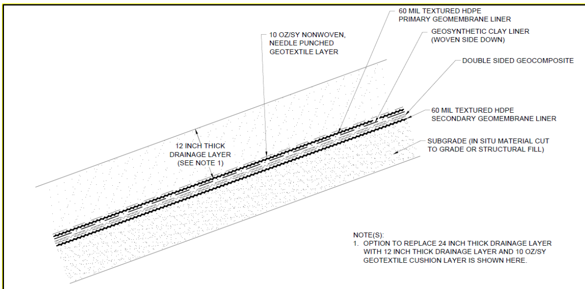
Figure 2: Cell 6 Liner System - Side Slope
