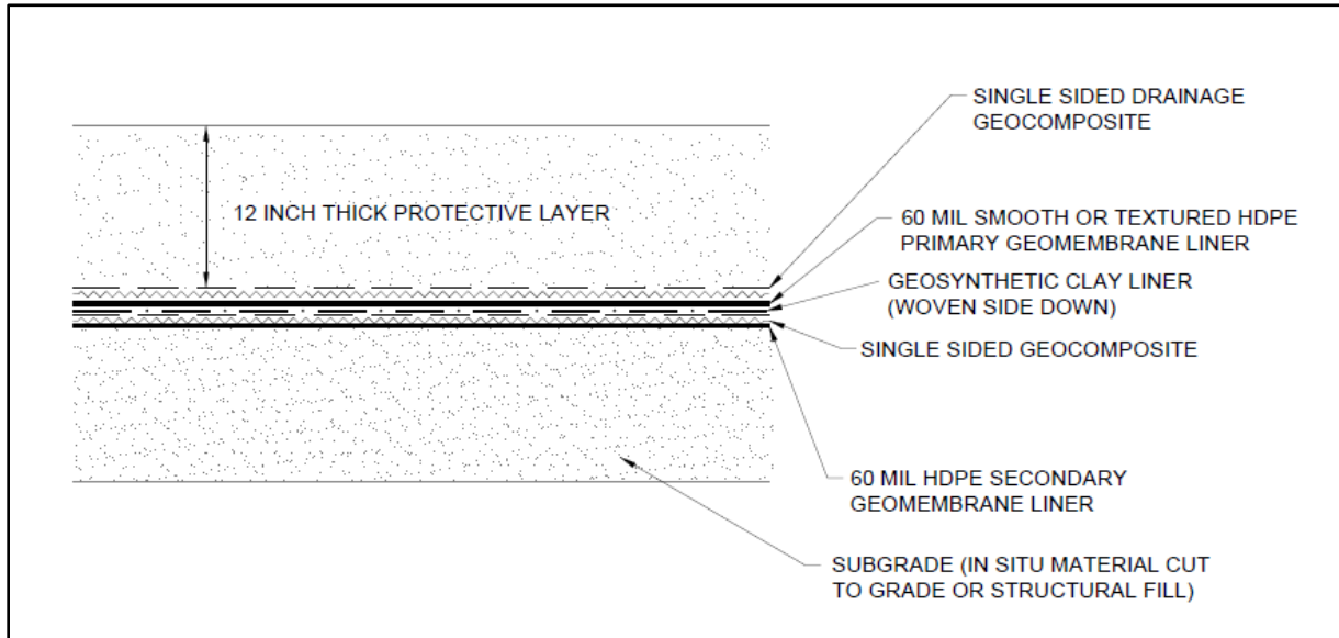
Figure 1: Cell 6 Liner System – Floor
